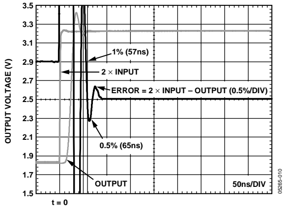
Figure 18. Settling Time
